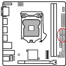
2-12 SATA Interface
