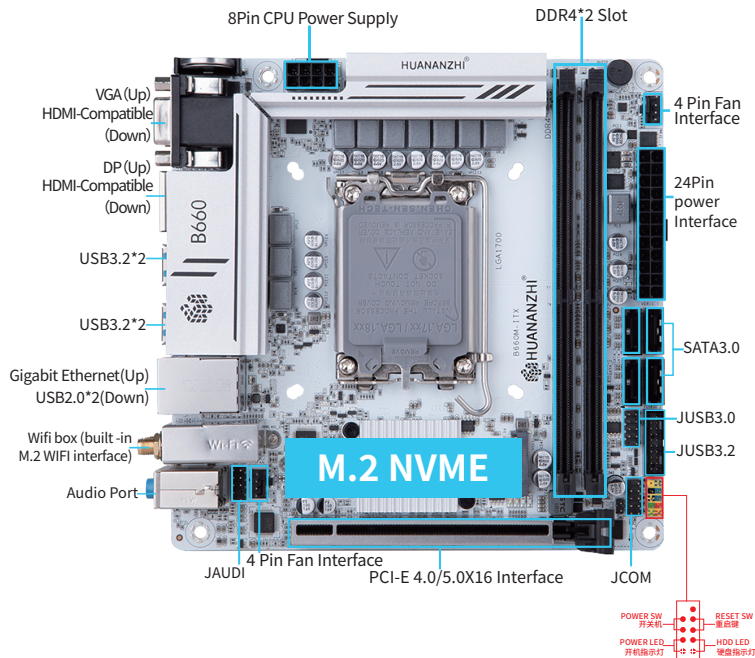
1-1 B660M-ITX MotherBoard Illustration
